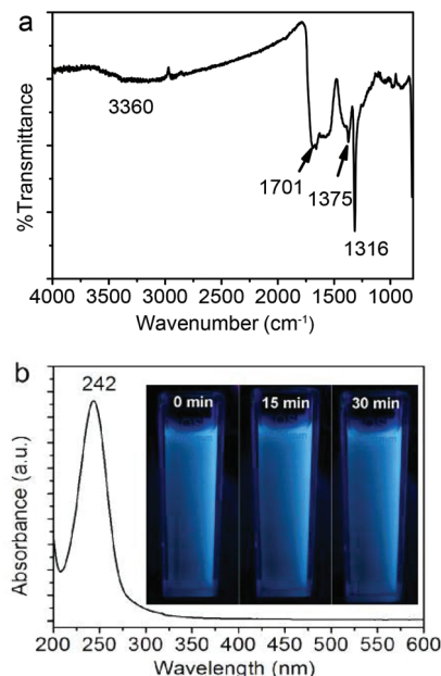
Fig. 3 (a) Typical FT-IR spectrum and (b) UV-Vis spectrum of the as-obtained \text{Fe}_3\text{O}_4\text{@C-CDs} NPs. The inset in (b) shows photographs of the aqueous dispersions of the \text{Fe}_3\text{O}_4\text{@C-CDs} NPs under UV light (365 nm) with different exposure times from 0 min to 30 min.
