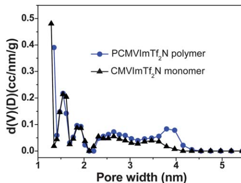
Fig. 3 Pore size distribution curves of nitrogen-doped micro/mesoporous carbons prepared from the IL monomer CMVImTf 2 N and the PIL polymer PCMVImTf 2 N at 600 °C under nitrogen (heating rate: 10 °C min -1 , kept at 600 °C for 1 h).
