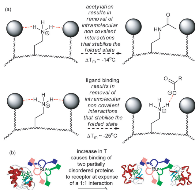
Fig. 4 Schematic depicting the basis of reduced T_m in cyt c (a) post covalent modification and binding to surface receptors results in structural loosening in order to maximise non-covalent contacts (b) a change in stoichiometry results on increasing the temperature and is promoted by binding of more disordered proteins.
