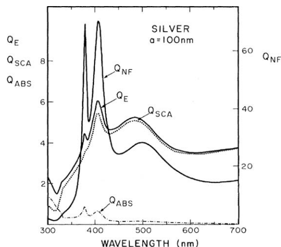
Fig. 9 Extinction, far-field scattering, and absorption efficiency (scale on the left side) compared with the near-field scattering efficiency (scale on the right side) for spheres with a = 100 nm immersed in water. (Reprinted with permission from ref. 41. Copyright 1981, American Physical Society.)
