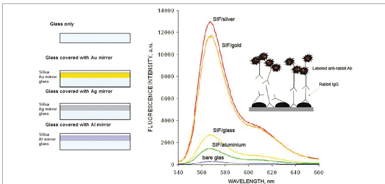
Fig. 47 Left: schematic of substrates with silver particles above a smooth metal film. Each substrate has silver particles on the silica. Right: emission spectra of Alexa Fluor 555®-labeled IgG on the substrates. (Reprinted with permission from ref. 143. Copyright 2007, Elsevier.)
