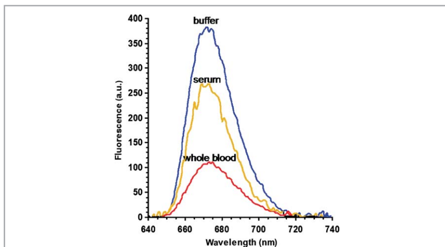
Fig. 46 Fluorescence spectra (SPCE) of the Alexa Fluor 647 ® -labeled anti-rabbit antibodies bound to the rabbit IgG immobilized on a 50 nm silver mirror surface observed in buffer, human serum, and human whole blood (KR configuration), a.u. = arbitrary units. (Reprinted with permission from ref. 142. Copyright 2005, Elsevier.)
