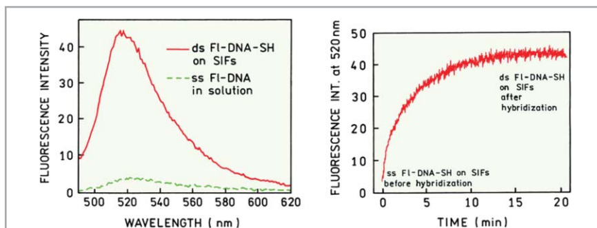
Fig. 18 Emission spectra and time-dependent intensity of a fluorescein-labeled oligomer upon binding to a complementary oligomer bound exclusively to an SIF. (Reprinted from ref. 85. Copyright 2003, with permission from Elsevier.)
