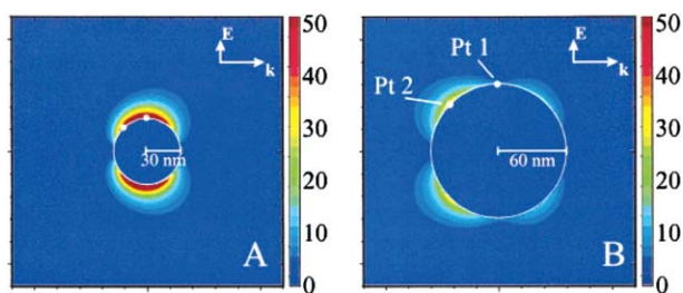
Fig. 10 Total electric field intensity near 60 nm (left) and 120 nm (right) diameter colloids calculated by the DDA method. 35 The light is propagating from left to right. (Reprinted with permission from ref. 35. Copyright 2003, American Chemical Society.)
