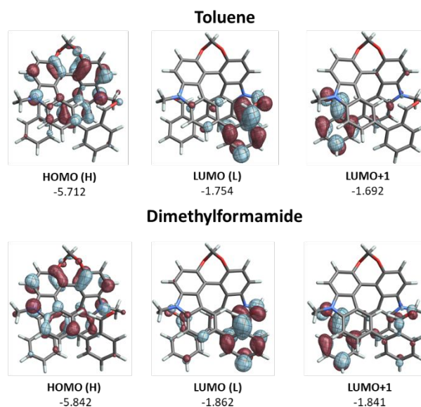
Figure 5. Isosurfaces ( \pm 0.04 au) of frontier Molecular Orbitals (MOs) for (+)-Hel-o-CHO in toluene (up) and dimethylformamide (down) with their
