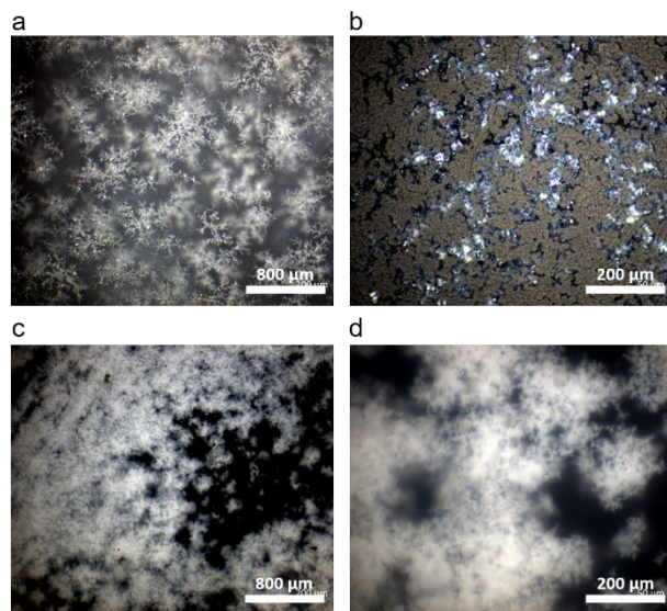
Figure 6. (a) and (b) Dendritic structures are seen in other locations of the same C_{10} sample along with the crystals shown in Figure 5. (c) (d) After annealing at 50 °C for 2 days the dendrites span the entire crystal domain and the spherulites are no longer visible.
