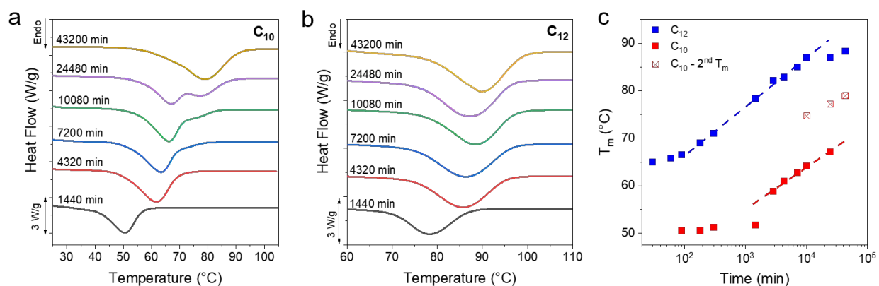
Figure 3. (a, b) DSC of C_{10} and C_{12} after long time crystallization at room temperature. A monotonic increase in the T_m is evident from the rightward shift of the melting curve. DSC data for less than 1 day of crystallization time can be found in Figure S2 . (c) A plot of T_m vs time shows similar slopes for the two networks. The 7, 17 and 30 day samples of C_{10} show two melting peaks, the lower one shown as solid squares and the higher peak as crossed squares.
