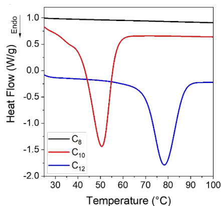
Figure 2. After 1-day of isothermal crystallization at room temperature, C_{10} and C_{12} show clear melting peaks whereas C_8 still exhibits no melting transition.
