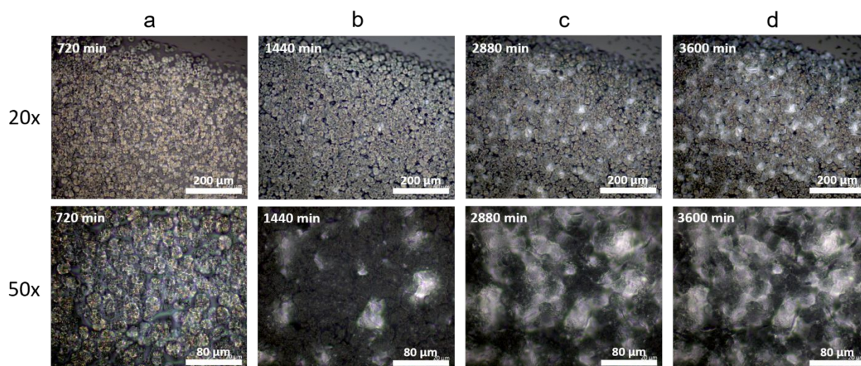
Figure 5. Cross polarization microscopy of C_{10} , crystallization at room temperature under ambient condition. We follow the evolution in crystal structure as a function of time (from left to right). (a) Initial formation of spherulites after 720 min of crystallization time. (b) A new crystal structure is
