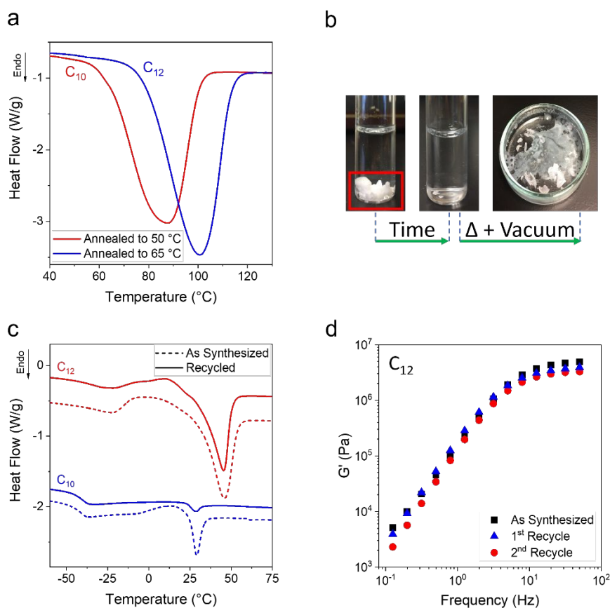
Figure 7. (a) DSC of the annealed samples. After annealing for 2 days an increase in T_m to 89 °C and 100 °C is observed for C_{10} and C_{12} respectively. (b) Networks were dissolved in ethanol and recovered by solvent evaporation. (c) DSC of as synthesized vs recycled C_{10} and C_{12} . The T_g and T_m of the recovered networks match the virgin networks. (d) Comparison of the rheology of recycled C_{12} and as synthesized C_{12} network indicates that there is minimal degradation in material properties.
