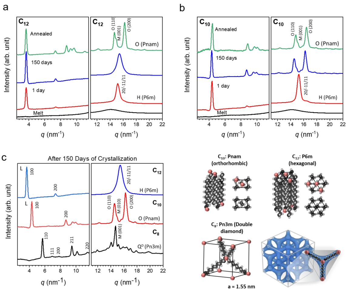
Figure 4. (a), (b) Room temperature WAXS patterns of C 10 and C 12 networks crystallized in a glove box. Samples were sandwiched and sealed between Kapton to prevent exposure to moisture. After 150 days of crystallization, samples were annealed at 50 °C (C 10 ) and 65 °C (C 12 ) for 2 days for the “annealed” data set. (c) A comparison of the WAXS patterns after 150 days of crystallization. (d) Schematic representation of the hexagonal ( P6m ), orthorhombic ( Pnam ) and double diamond ( Pn3m ) crystal lattices adopted by the C 12 , C 10 , and C 8 polymers, respectively.
