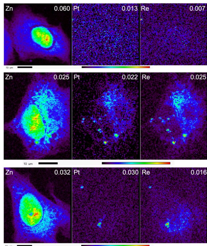
Fig. 2 X-ray fluorescence elemental distribution maps (Zn, Pt and Re) of: (top) untreated HeLa cells; (middle) HeLa cells treated with 8.5 μM OxaliPtRe in media in the dark for 7 h; (bottom) HeLa cells treated with 8.5 μM OxaliPtRe in media for 7 h, including irradiation at 365 nm for 1 h, starting 3 h into the treatment. The maximal elemental area density (units of μg cm -2 ) is given in each map. The nucleus is evident in the zinc-rich region of each cell.
