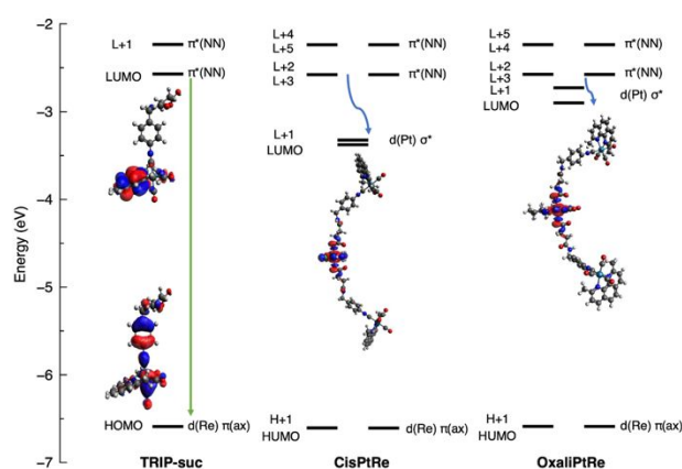
(HOMO, HOMO–1) of TRIP-suc . The presence of these Pt-based d orbitals gives rise to additional excited states that reside lower in energy than the optically active MLCT state of TRIP-suc , as calculated by TD-DFT (Fig. S28, ESI † ). Of significance to the experimentally observed photoreduction pathways of CisPtRe and OxaliPtRe , several of these intermediary excited states have metal-to-metal charge transfer (MMCT) character, whereby an electron transitions from the Re “t 2g -like” d orbital into a Pt “e g -like” \sigma^* orbital. Although these MMCT excited states have very low oscillator strengths and are not likely to be directly accessed via irradiation with light, population of the high oscillator strength MLCT states of TRIP-suc by photoexcitation followed by photoinduced electron transfer to these MMCT states is energetically viable. Because these MMCT excited states require population of Pt \sigma^* orbital, dissociation of the axial TRIP-suc ligands, as observed experimentally, will occur. Assuming that this electron transfer occurs in the “non-inverted Marcus region”, 37 the lower photoreduction quantum yield of OxaliPtRe compared to
