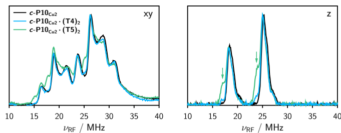
Fig. 4 Comparison of the ^{14}\text{N} Davies ENDOR spectra of all three samples recorded at field positions corresponding to the xy (left) and z (right) orientations in frozen toluene- d_8 at 15 K. The green arrows indicate the additional nitrogen hyperfine coupling observed for \mathbf{c-P10Cu}_2\cdot(\text{T5})_2 .
