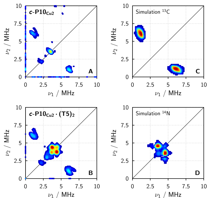
Fig. 5 Experimental HYSCORE spectra for c-P10Cu 2 ( A ) and c-P10Cu 2 ·(T5) 2 ( B ) recorded in regular toluene at 15 K and simulations of individual contributions to the experimental spectra using EasySpin for a ^{13}\text{C} nucleus with hyperfine couplings of 4.0 5.0 and 7.2 MHz for A_x , A_y , and A_z ( C ) and a ^{14}\text{N} nucleus with hyperfine couplings of [-1.15 -1.14 -0.29] MHz and nuclear quadrupole couplings of [0.80 1.30 -2.10] MHz ( D ).
