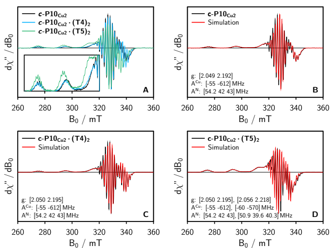
Fig. 3 A: Comparison of the baseline corrected continuous wave EPR spectra of the investigated samples at 100 K recorded at X-band in frozen toluene- d 8 . B-D: Numerical simulations of the experimental data as explained in the main text. The simulation parameters are indicated in the figure. The relative contribution of the second component in the simulation for c-P10Cu 2 ·(T5) 2 amounts to \approx 40\% .
