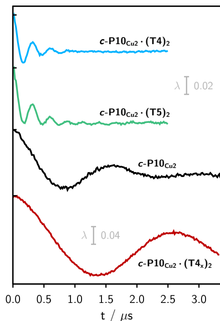
Fig. 6 Experimental background-corrected DEER traces for c-P10 Cu2 ( T4 ) 2 , c-P10 Cu2 ( T5 ) 2 and c-P10 Cu2 (from top to bottom) recorded at 15 K in toluene- d 8 . The bottom panel shows the DEER trace of a complex of c-P10 Cu2 with an isomer of T4 , referred to as T4 x as discussed in the main text. The modulation depth scale of 2% refers to the upper three traces, whereas the scale of 4% applies to the bottom trace.
