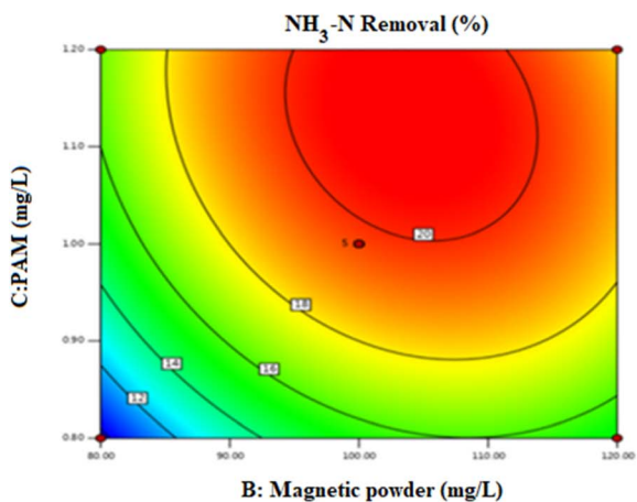
Fig. 5 Effect of the interaction of various factors on the ammonia nitrogen removal efficiency.
