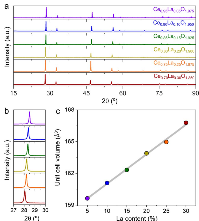
Fig. 1 Lanthanum doping expands the ceria lattice while preserving fluorite structure. (a) XRD patterns of Ce 1-x La x O 2-δ ( x = 0.05 – 0.30 ), all indexed to the fluorite phase; (b) zoom-in of primary diffraction peaks shows peak shifts with increasing La content; and (c) unit cell volume increases linearly with La content, confirming solid solution behavior by Vegard's law.
