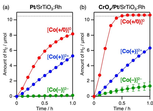
Fig. 3 Time courses of H 2 evolution using (a) Pt- or (b) CrO x /Pt-loaded SrTiO 3 :Rh (10 mg) in an aqueous solution (70 mL, pH 3.5) containing [\text{Co}(+)]^{2+} , [\text{Co}(+/0)]^{+0} , or [\text{Co}(-)]^{2-} (0.3 mM each) as an electron donor under visible-light irradiation ( \lambda = 430 \text{ nm} ). The broken lines show the upper limit of H 2 evolution expected from the amount of Co II species added to the solutions.
