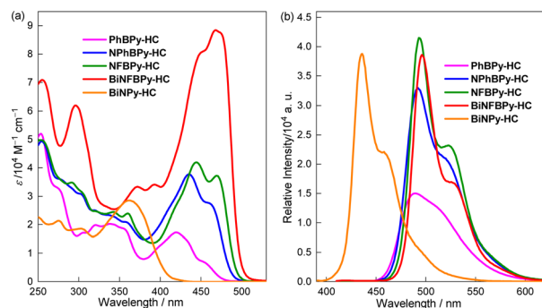
Fig. 3 (a) UV/vis absorption ( c = 2.0 \times 10^{-5} M) and (b) fluorescence spectra ( c = 1.0 \times 10^{-5} M and \lambda_{\text{ex}} = 400 nm) of B ← N Lewis pair-fused [6]helicenes in cyclohexane.
