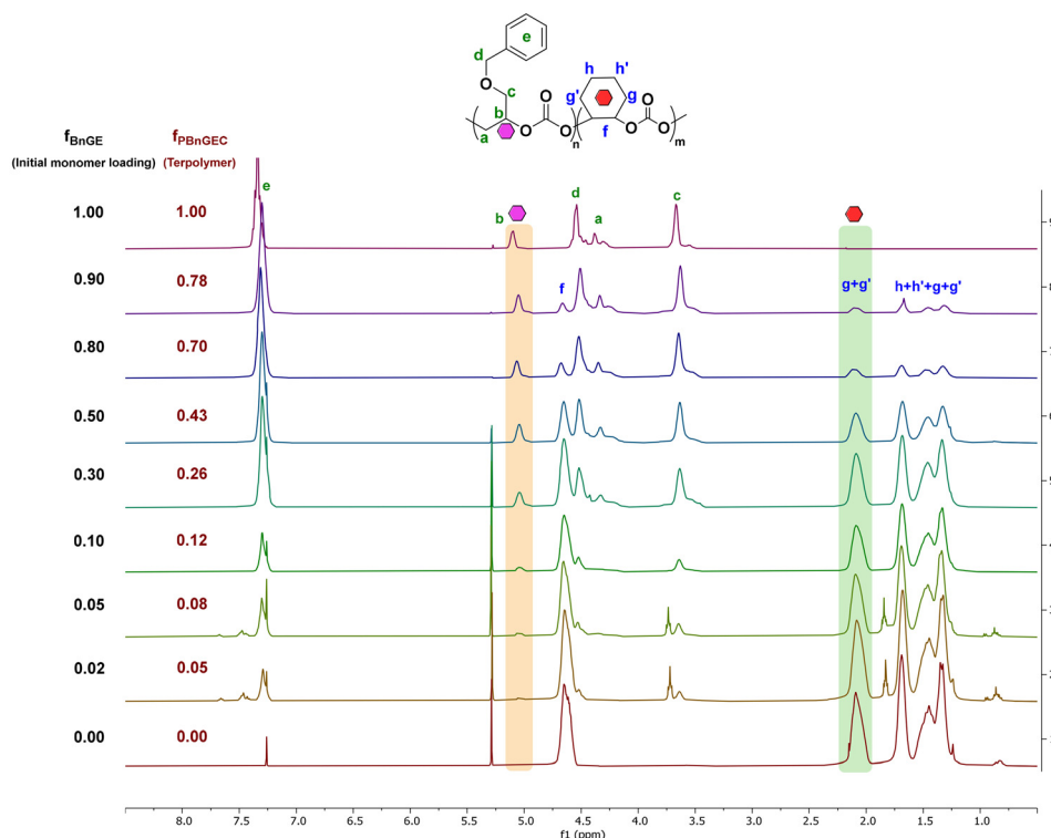
Fig. 4 ^1\text{H} NMR spectra (400 MHz, \text{CDCl}_3 , 23 ^\circ\text{C} ) of P(BnGEC-co-CHC) terpolymers synthesized with the \text{BEt}_3 /PPNCl system at various BnGE/CHO loadings (Table 3).
