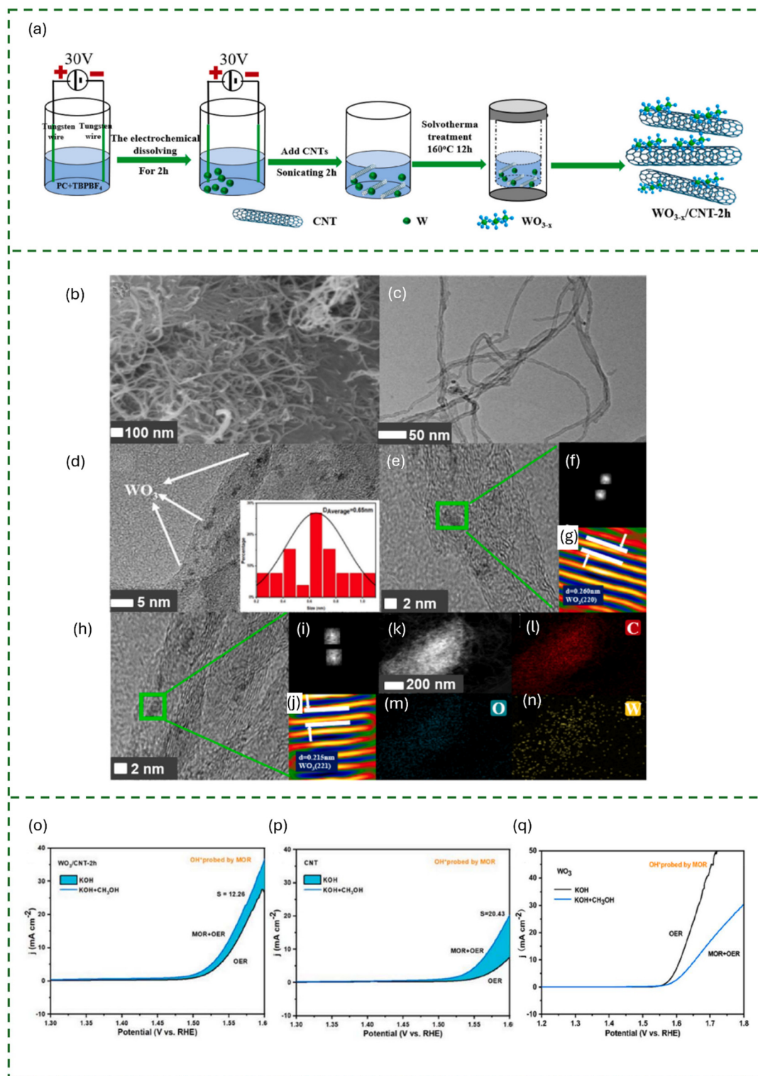
Fig. 8 (a) A schematic illustration of the synthesis process of \text{WO}_{3-x}/\text{CNT} -2 h. (b) SEM images of \text{WO}_{3-x}/\text{CNT} -2 h, (c–j) TEM images of \text{WO}_{3-x}/\text{CNT} -2 h, (k) HAADF-STEM images of \text{WO}_{3-x}/\text{CNT} -2 h, and elemental mappings of (l) carbon, (m) oxygen, and (n) tungsten. (o) LSV curves for MOR and OER on \text{WO}_{3-x}/\text{CNT} -2 h, (p) CNT, and (q) \text{WO}_3 in 1 M KOH and 1 M KOH + \text{CH}_3\text{OH} at a scan rate of 50 \text{mV s}^{-1} . 95 Figures a–q reprinted from ref. 95 Int. J. Hydrogen Energy , 2025, 127 , 903–911, with permission from Elsevier, copyright 2026.
