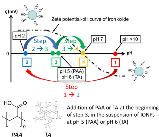
Fig. 1 Schematic of the coating protocol with PAA and TA. The dashed line represents a typical zeta potential-pH curve of naked IONPs. Step 1 → 2: quick adjustment from pH > 10 to 2 to turn the naked IONPs \zeta positive. Step 2 → 3: adjustment from pH 2 to a value above surfactant pK_a (deprotonated, thus negatively charged) and below the IO IEP (naked IONPs with slightly positive \zeta ). Step 3 → 4: addition of the surfactant (here, PAA or TA) and then adjustment to pH 7.
