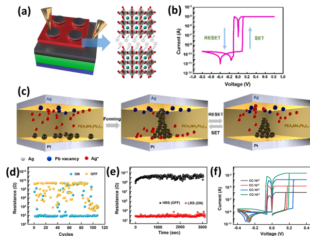
Fig. 3 (a) Schematic representation of the structure of the resistive switching memory device and the resistive switching materials (PEA) 2 MA 3 Pb 4 I 13 . (b) I – V characteristics of an Ag/(PEA) 2 MA 3 Pb 4 I 13 /Pt device derived from five sequential voltage sweeps. (c) Schematic representation of the ECM mechanism. (d) Endurance characteristics for the (PEA) 2 MA 3 Pb 4 I 13 memory device. (e) Retention characteristics of an Ag(PEA) 2 MA 3 Pb 4 I 13 /Pt device under four distinct CC. Reproduced with permission. 72 Copyright 2024, Elsevier.
