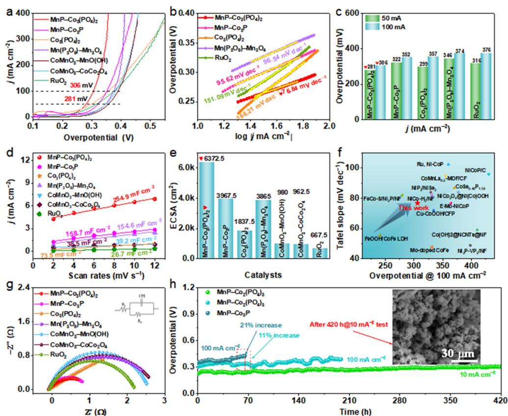
Fig. 4 (a) LSV polarization curves, (b) Tafel slopes, (c) summary of overpotentials (at 50 and 100 mA cm -2 ) in 1.0 M KOH, (d) C dl and (e) summary of ECSA of the designed catalysts. (f) Comparison of overpotentials (at 100 mA cm -2 ) and Tafel slopes for various state-of-the-art OER catalysts. (g) Electrochemical impedance spectroscopy of prepared catalysts. (h) Chronopotentiometry of MnP-Co 3 (PO 4 ) 2 /NF (at 10 and 100 mA cm -2 ) and MnP-Co 3 P/NF (at 100 mA cm -2 ) (the inset shows the morphology of MnP-Co 3 (PO 4 ) 2 /NF after stability at 10 mA cm -2 ).
