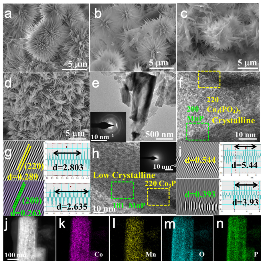
Fig. 2 SEM images of (a) \text{CoMnO}_3\text{-MnO(OH)/NF} , (b) \text{CoMnO}_3\text{-CoCo}_2\text{O}_4\text{/NF} , (c) \text{MnP-Co}_3(\text{PO}_4)_2\text{/NF} and (d) \text{MnP-Co}_3\text{P/NF} . (e) TEM image/SAED image (inset), (f) HR-TEM image, and (g) the intensity profile of corresponding areas of the \text{MnP-Co}_3(\text{PO}_4)_2\text{/NF} . (h) HR-TEM image/SAED image (inset) and (i) the intensity profile of corresponding areas of the \text{MnP-Co}_3\text{P/NF} . (j) HAADF-STEM image and (k–n) elemental mappings (Co, Mn, O, and P) of the \text{MnP-Co}_3(\text{PO}_4)_2\text{/NF} .
