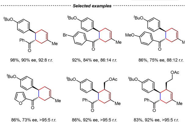
Scheme 51 A new \text{Fe}(\text{III}) photocatalyst consisting of a chiral phosphoramidate anion and an achiral bidentate ligand.
