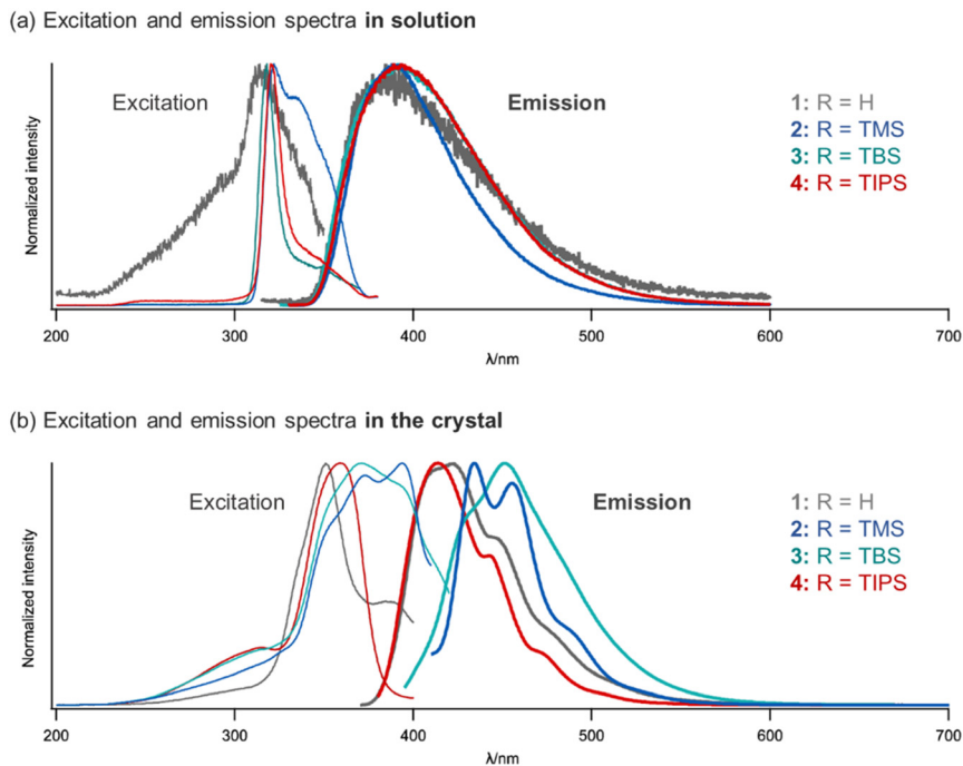
Fig. 4 Excitation and emission spectra of 1–4 in (a) dilute chloroform solutions (concentration: 10^{-3} mol L -1 for both spectra) and (b) the crystalline state.
