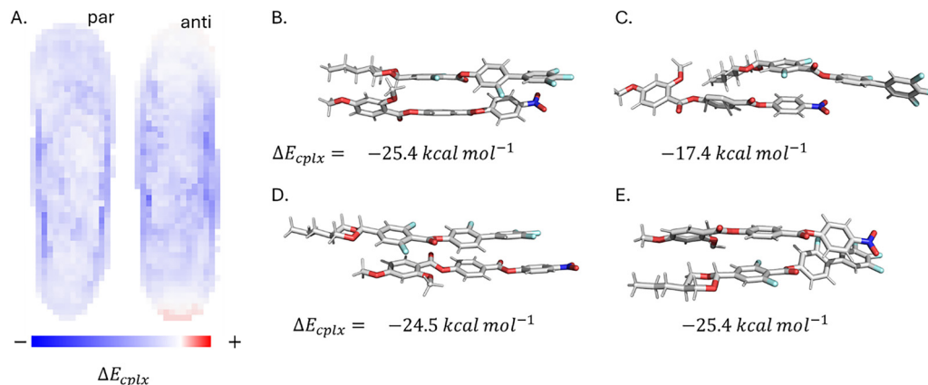
Fig. 9 (A) Bimolecular potential energy surfaces for the RM734/DIO system in parallel and antiparallel configurations. Optimised minimum energy configurations of RM734/DIO (B)–(E). \Delta E_{cplx} is the counterpoise complexation energy at the DFT B97D3/cc-pVTZ level.
