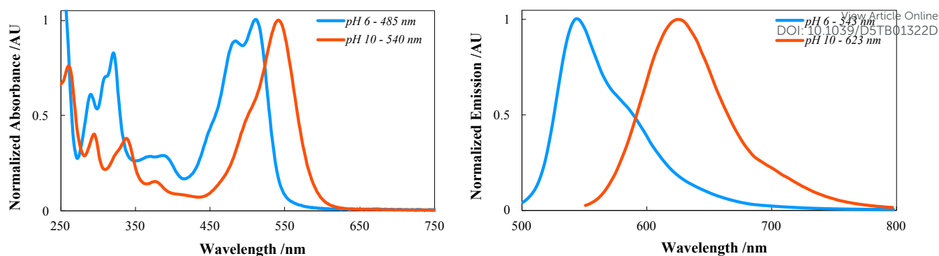
Figure 1. Normalized absorption and emission spectra of SNAFL-C at pH 6 (naphthol, PBS buffer, \lambda_{ex} = 485 nm) and pH 10 (naphtholate, carbonate/bicarbonate buffer, \lambda_{ex} = 540 nm)
