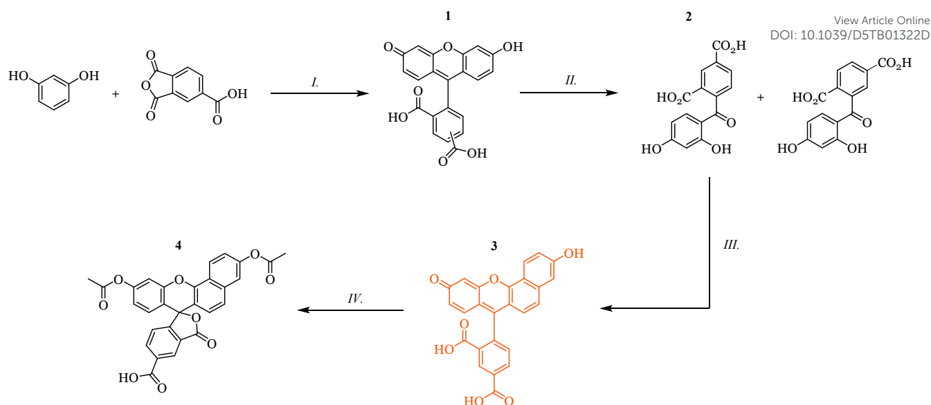
Scheme 3. Synthesis and protection of single isomer SNAFL-C ( 3 ). I. MeSO 3 H, 80°C, 18 h. II. 50% NaOH (aq.), 95°C, 24 h. III. 1,6-naphthalene diol, MeSO 3 H/TFA, RT, 24 h. IV. Acetic anhydride, pyridine, 110°C, 1 h.
