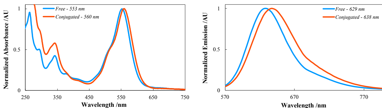
Figure 3. Normalized absorption and fluorescence emission spectra ( \lambda_{ex} = 560 nm) of SNAFL-C and conjugate \mu_2 in ethanolic potassium hydroxide solution
