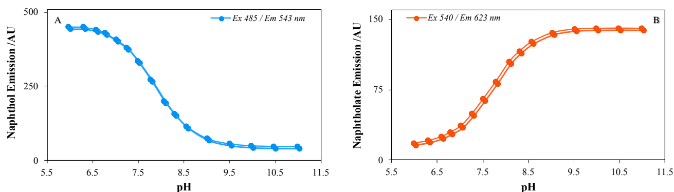
Figure 2. Ratiometric emission of SNAFL-C with A) Naphthol excited at 485 nm and monitored at 543 nm B) Naphtholate excited at 540 nm and monitored at 623 nm
