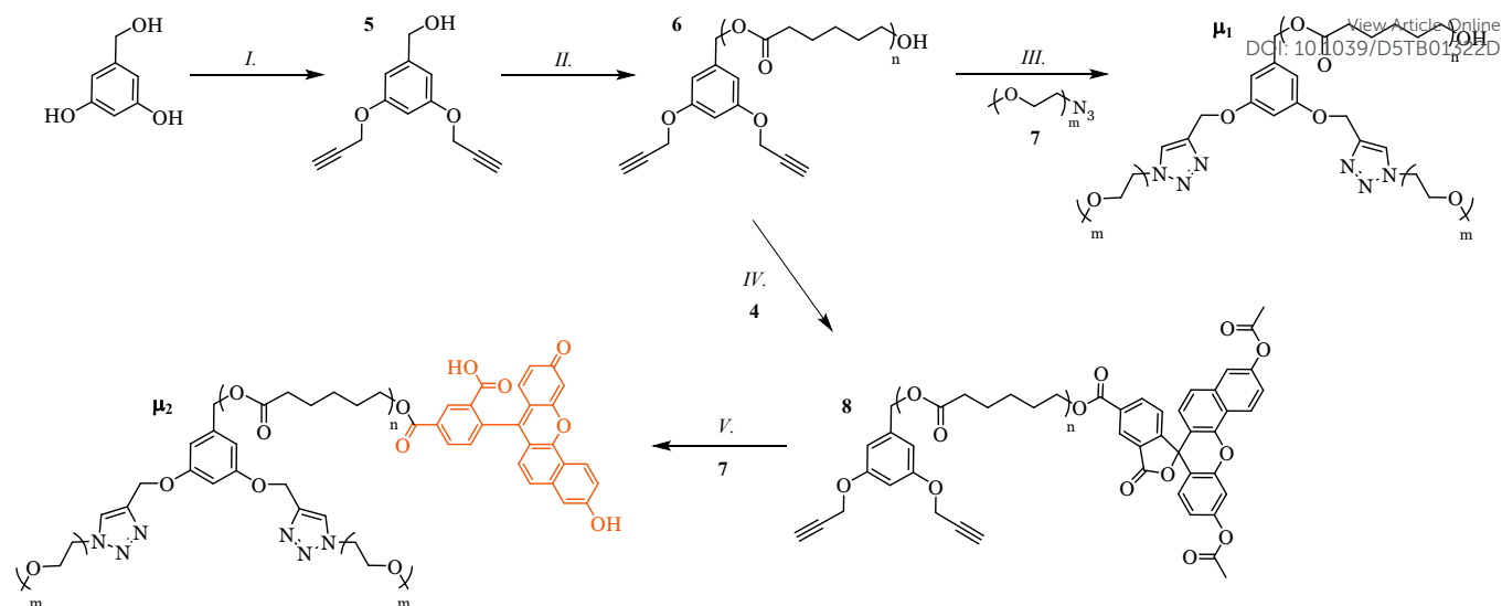
Scheme 4. Synthesis of miktoarm polymers \mu_1 (unlabelled PEG 2 -PCL) and \mu_2 (fluorescent PEG 2 -PCL-SNAFL). I. Propargyl bromide, K 2 CO 3 , 18-Crown [6], acetone, 60 °C, 18 h. II. \epsilon -Caprolactone, Tin(II) ethyl hexanoate, toluene, 110 °C, 18 h. III. mPEG 2000 -N 3 (7), CuBr, N,N'-PMDETA, DMF, 40 °C, 24 h. IV. SNAFL-Diacetate (4), DCC/DMAP, DCM, 0 °C – RT, 48 h. V. CuBr, N,N'-PMDETA, DMF, 40 °C, 24 h.
