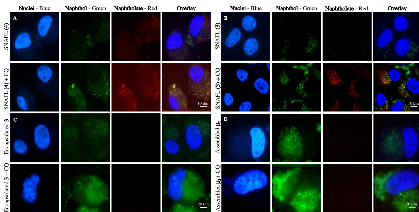
Figure 7. Detection of A) Free SNAFL-C (compound 3 ), B) SNAFL diacetate (compound 4 ), C) Encapsulated SNAFL-C, and D) Assembled conjugate \mu_2 in human glioblastoma cells. Cells were treated with chloroquine (CQ, 25 \mu M) for 24 hours where appropriate. 1.5 \mu M of the selected fluorophore was added 30 minutes prior to imaging. Species were detected using fluorescent live imaging (GFP green and Cy5 filters); nuclei were labelled with Hoechst 33342 blue.
