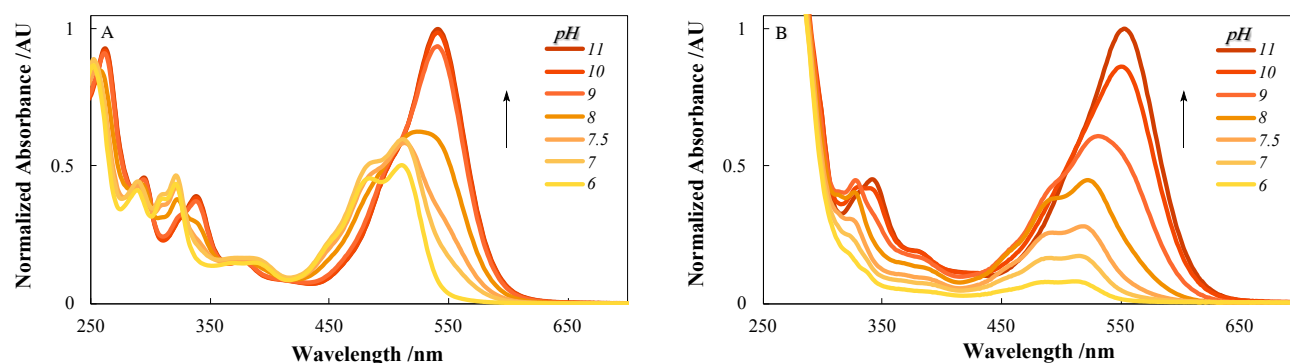
Figure 4. Absorption spectra of A) Physically encapsulated SNAFL-C and B) Assembled conjugate \mu_2 over pH range 6 - 11
