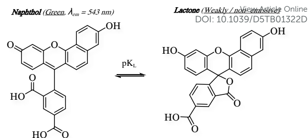
Scheme 5. Equilibrium between SNAFL-C naphthol and ring closed lactone species
