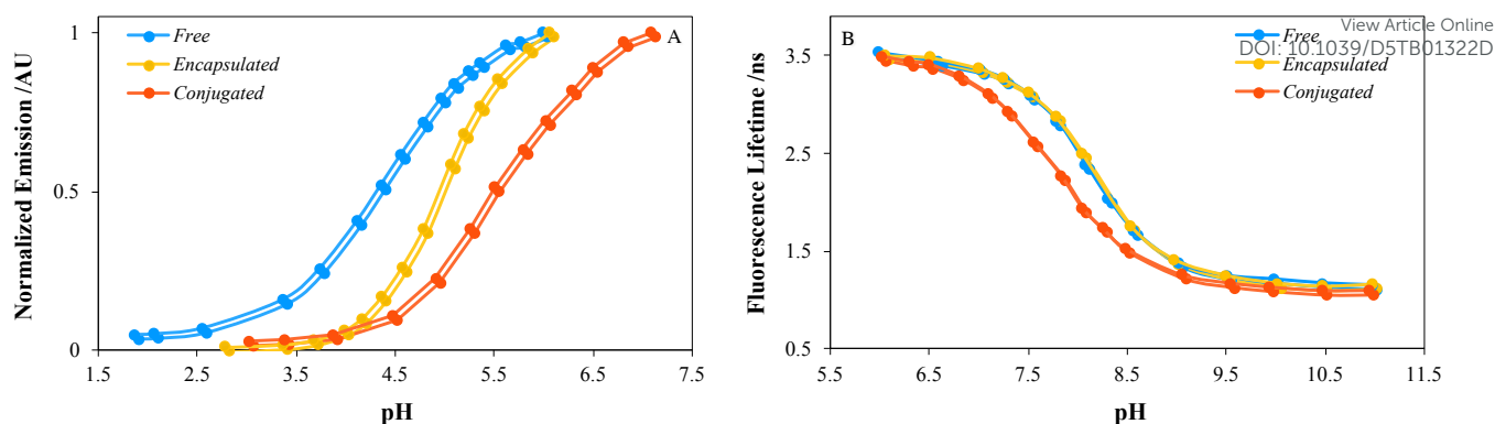
Figure 6. A) Decay of naphthol fluorescence in the acidic pH regime demonstrating formation of the SNAFL-C lactone; and B) Fluorescence lifetimes of free SNAFL-C, encapsulated SNAFL-C, and assembled conjugate \mu_2
