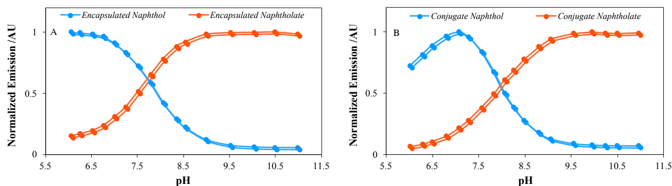
Figure 5. Visualized equilibrium between A) Encapsulated SNAFL-C naphthol ( \lambda_{ex} = 485 nm, \lambda_{em} = 543 nm) and naphtholate ( \lambda_{ex} = 540 nm, \lambda_{em} = 623 nm) in comparison to B) Assembled \mu_2 -naphthol ( \lambda_{ex} = 485 nm, \lambda_{em} = 549 nm) and naphtholate ( \lambda_{ex} = 540 nm, \lambda_{em} = 635 nm)
