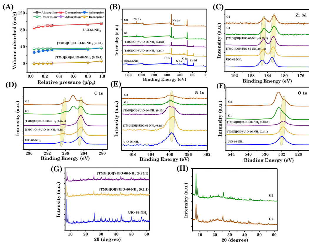
Fig. 1 (A) \text{N}_2 adsorption–desorption isotherms of UiO-66- \text{NH}_2 and UiO-66- \text{NH}_2 -IL composites; (B) wide-scan XPS spectra; high-resolution XPS spectra of (C) Zr 3d, (D) C 1s, (E) N 1s, and (F) O 1s; PXRD patterns of (G) MOF and IL@MOF composites and (H) IL@MOF composite-based hydrogels.
