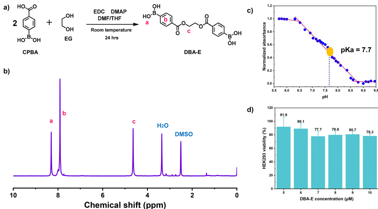
Fig. 2 For a new DBA-E phenyldiboronic acid crosslinker: synthesis exploring an EDC-mediated coupling reaction (a), ^1\text{H} NMR spectrum in DMSO- d_6 (b), spectroscopic titration curve of normalized absorbance at \lambda = 285 nm over a pH range of 5.5–9.5 (c), and viability of HEK293 cells incubated for 24 h using a resazurin reduction assay (d).
