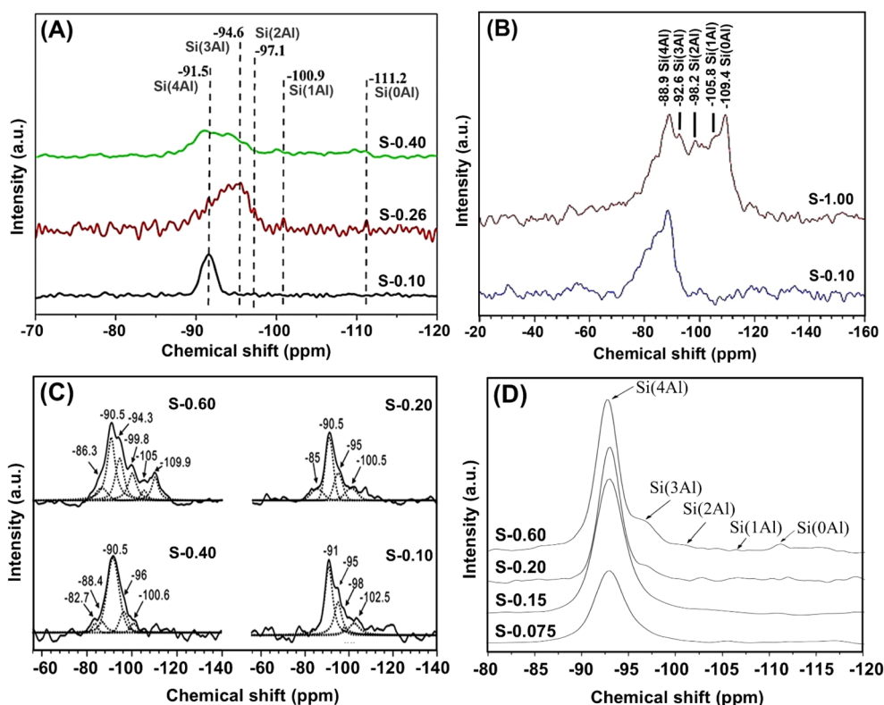
Fig. 30 ^{29}\text{Si} NMR spectrum for SAPO-34 (S- x ) samples, where x stands for different \text{SiO}_2/\text{Al}_2\text{O}_3 ratios. (A) Reproduced from ref. 296 with permission from Elsevier, Copyright 2019. (B) Reproduced from ref. 280 with permission from Elsevier, Copyright 2008. (C) Reproduced from ref. 299 with permission from Royal Society of Chemistry, Copyright 2014. (D) Reproduced from ref. 300 with permission from Elsevier, Copyright 2008.
