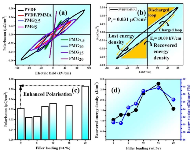
Fig. 8 P - E hysteresis loop of (a) the composite film and (b) PVDF/PMMA blend. (c) Remnant polarization ( P_r ) and (d) recovered energy density ( W_1 ) and storage efficiency ( \eta ) with different wt% GMHs at ambient temperature.
