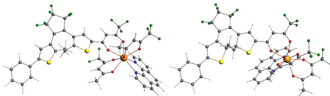
Fig. 8 Representation of the DFT-optimized 3\text{Yb}_o\text{-}S_0 (left) and 3\text{Yb}_c\text{-}S_0 (right) model compounds.
