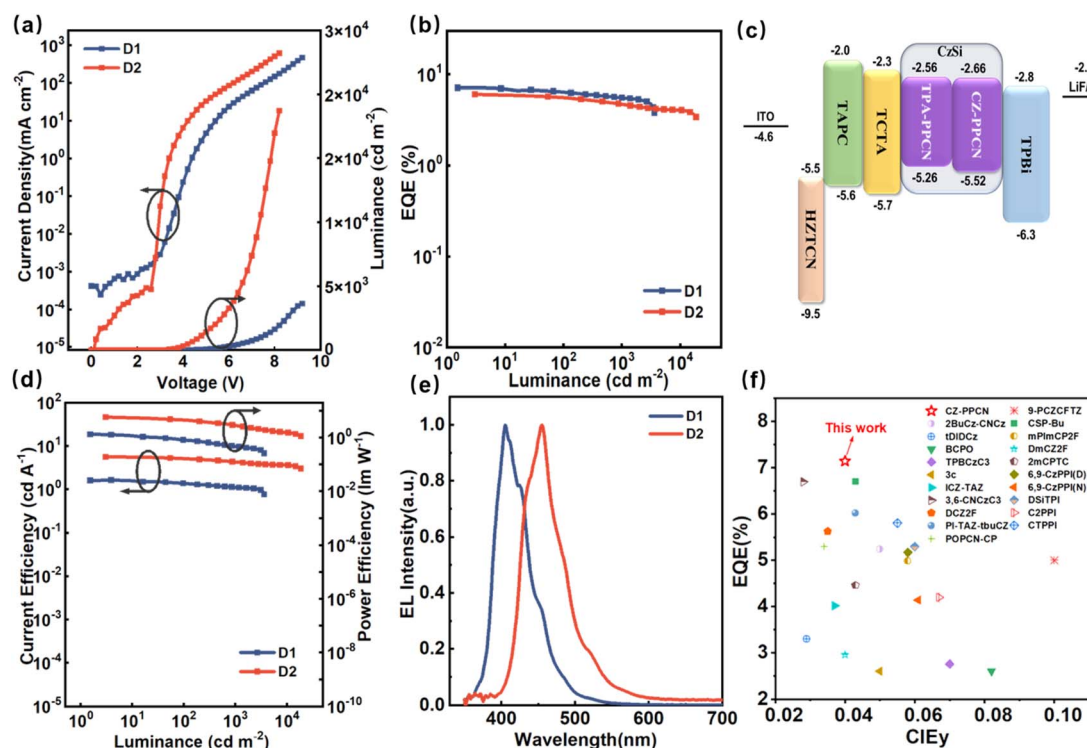
Fig. 5 (a) Current density–voltage–luminance curves, (b) EQE–luminance curves, (c) device structures and energy levels, (d) current efficiency–luminance–power efficiency curves, and (e) EL spectra of doped OLEDs with 25 wt% emitters (CZ-PPCN and TPA-PPCN for D1 and D2). (f) Performance comparison of NUV electroluminescent devices (EL peak \leq 410 nm) based on the HLCT mechanism ("N" for a non-doped device and "D" for a doped device).
