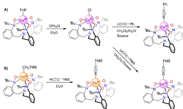
Fig. 2 Syntheses of (A) \text{Ce}^{\text{IV}} -alkynyl complexes ( 1-Ce Ph and 1-Ce TMS ) and (B) \text{Th}^{\text{IV}} -alkynyl complex ( 1-Th TMS ).
