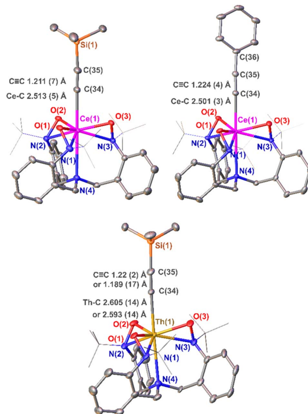
Fig. 3 X-ray crystal structures of 1-Ce TMS , 1-Ce Ph and 1-Th TMS . Thermal ellipsoids were plotted at a 30% probability level. For clarity, hydrogens and solvent molecules in the crystal structure are omitted; tert -butyl groups are displayed in wireframe.
