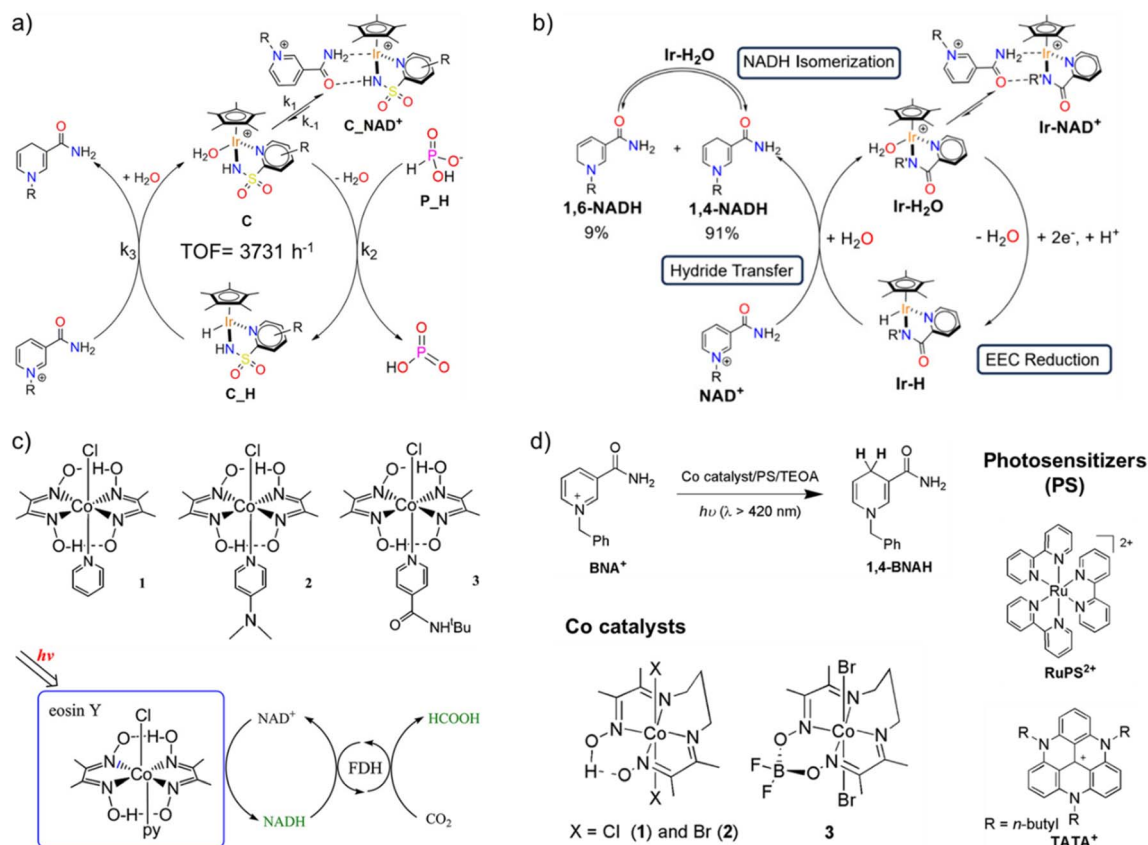
Fig. 8 Various electron mediators for regioselective regeneration of 1,4-NADH. (a) Schematics showing 1,4-NADH regeneration using iridium-pyridine-2-sulfonamide catalyst with phosphonic acid as the hydride source. Here, R = H , 4- CF_3 , or 6- NH_2 , out of which R = 6-NH_2 yields the highest TOF of 3731\text{ h}^{-1} at 313\text{ K} . Adapted with permission from ref. 89. Copyright 2020 American Chemical Society. (b) Schematic showing the mechanism of NADH regeneration using [Cp^*Ir(R'-pica)Cl] ( pica = R' -picolinamidate, R' = H and Me ) electron mediator. A rapid equilibrium was established between 1,4-NADH and 1,6-NADH in 91 : 9 ratio. Adapted with permission from ref. 90. Copyright 2024 American Chemical Society. (c) Structures of earth-abundant cobaloximes complexes for 1,4-NADH regeneration in presence of eosin Y as the light-harvesting moiety. The regenerated 1,4-NADH was coupled to enzymatic dark cycle to reduce CO_2 to formic acid. Adapted with permission from ref. 95. Copyright 2012 American Chemical Society. (d) Selective regeneration of 1,4-BNAH, a synthetic analogue of 1,4-NADH, in presence of cobalt diamine-dioxime complexes under visible light. Adapted with permission from ref. 97 Copyright 2020 The Royal Society of Chemistry.
