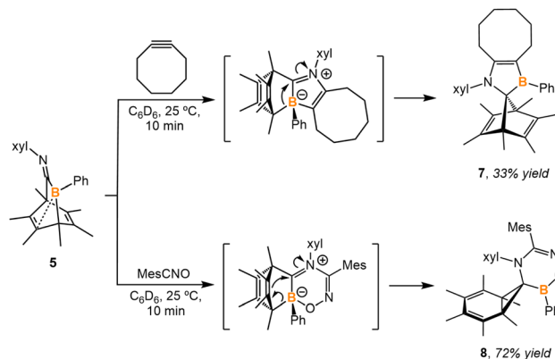
Scheme 4 Treatment of compound 5 with cyclooctyne and mesityl nitrite N-oxide.
