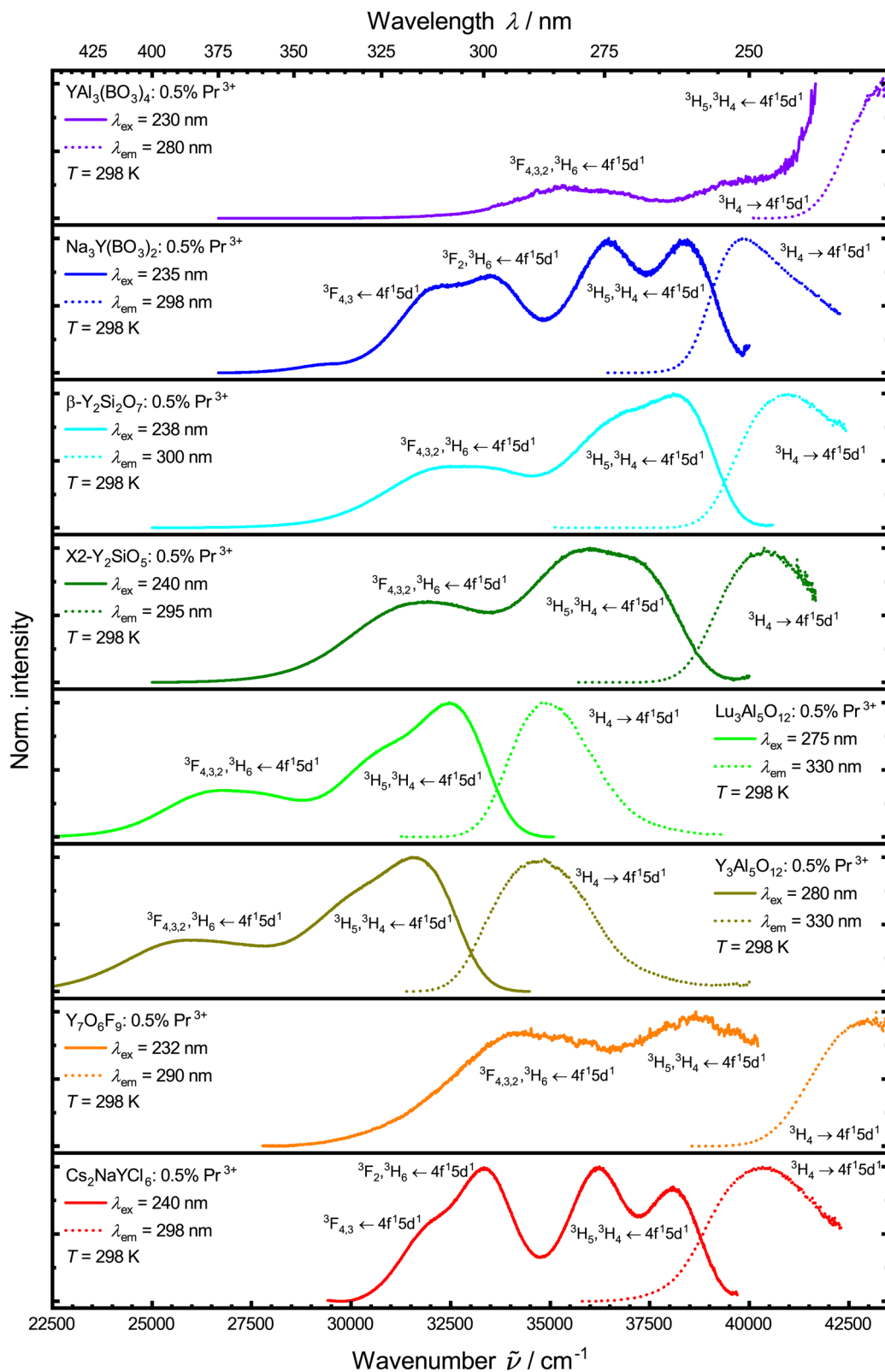
Fig. 5 Normalized photoluminescence emission (solid lines) and excitation spectra (dotted lines) of the synthesized samples at 298 K in UV range showing emission and excitation of 4f 1 5d 1 states. Spectra were measured against wavelengths and converted to wavenumbers using a Jacobian transformation. 99
