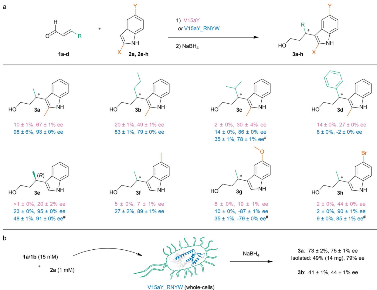
Scheme 2 (a) Substrate scope of the enantioselective vinylogous FC-alkylation catalysed by V15aY and V15aY_RNYW. Reaction conditions (unless otherwise noted): V15aY variant (60 \mu M dimer concentration), 1a–d (5 mM), 2a, 2e–h (1 mM) in MES buffer (20 mM, pH 5.5), containing NaCl (150 mM) and DMF (8% v/v) in a total volume of 300 \mu L, continuously inverted for 16 h at 8 ^{\circ} C. For 3a–d and 3f–h , ee is assigned relative to the enantiomer obtained with V15aY, in which the “–” symbol represents the opposite enantiomer. For 3e , absolute configuration is assigned by comparison of order of elution on HPLC with the literature and previous work. 16,42 # Performed using 25 mM 1 , see Table S5† for results of reactions performed at 25 ^{\circ} C. (b) Whole-cell catalysis and application on millimolar scale. Reaction conditions: washed whole-cells expressing V15aY_RNYW (6 OD 600 units), 1a/1b (15 mM), 2a (1 mM) in MES buffer (20 mM, pH 5.5), containing NaCl (150 mM) and DMSO (8% v/v) in a total volume of 300 \mu L, continuously inverted for 21 h at 8 ^{\circ} C. Results are based on at least three experiments, using two or more independently produced batches of protein, or three independent cultures of whole-cells. Errors are the standard deviation of the results. See ESI† sections 9 and 11 for more details.
