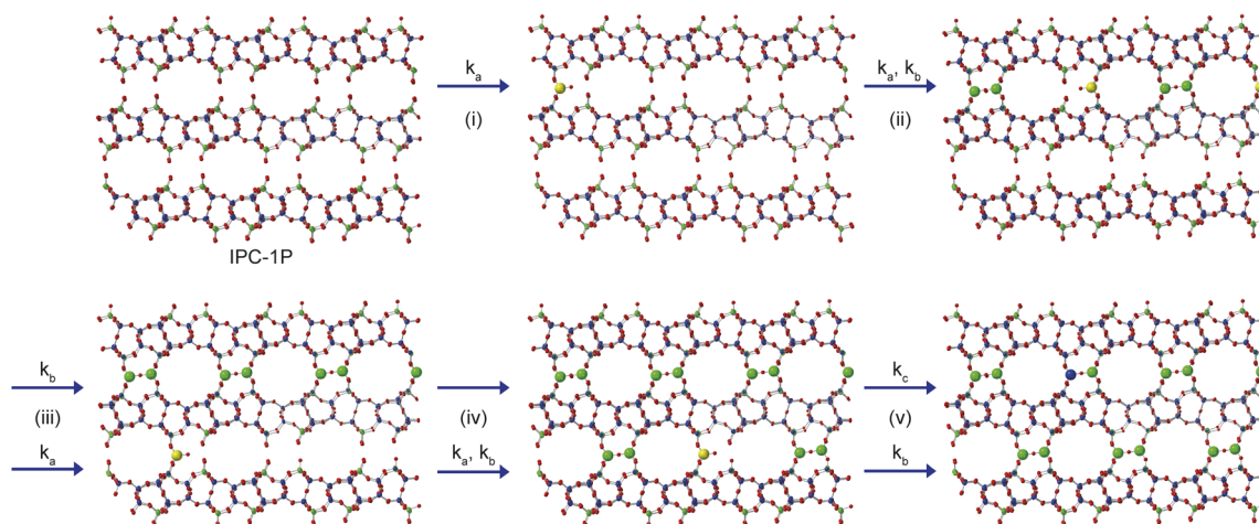
Fig. 7 Schematic showing the early stages of the mechanism for the formation of IPC-2P by sequential intercalation of \text{Si(OH)}_4 into IPC-1P. Steps (i) and (ii) show the loss of a to initially form b , and subsequently c , and steps (iii) and (iv) involve further reaction with \text{Si(OH)}_4 within additional layers to form a solid that contains a mixture of b and c . Step (v) contains the much slower reaction to form d in one layer, along with the simultaneous faster formation of c elsewhere. Structures a , b , c and d are defined in Fig. 5. Oxygen atoms are shown in red, and \text{Q}^2 , \text{Q}^3 and \text{Q}^4 Si atoms in yellow, green and blue, respectively.
