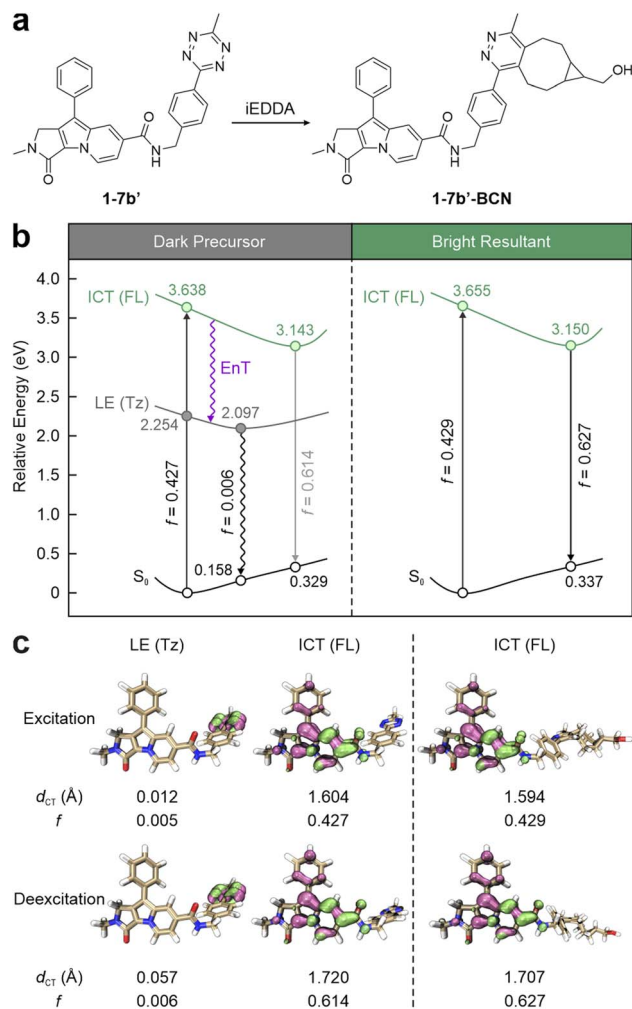
Fig. 2 (a) Molecular structures and (b) photophysical processes with (c) the corresponding hole–electron distributions, charge transfer distances ( d_{cr} ), and oscillator strength ( f ) values for different states of 1-7b' (left) and 1-7b'-BCN (right) in ethanol (EtOH). Hole – highlighted in mauve; electron – highlighted in green; FL – fluorophore; Tz – tetrazine; S_0 – ground state; LE – locally excited; ICT – intramolecular charge transfer. Reproduced with permission from ref. 53. Copyright 2023, The Royal Society of Chemistry.
