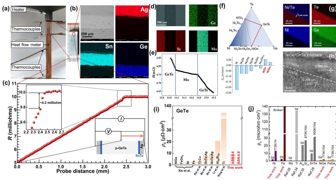
Fig. 23 (a) Experimental setup for the device efficiency measurement. (b) EDS mapping of the contacts. (c) Room-temperature contact resistance using a line scanning technique. 34 (d) SEM image and EDS elemental mapping performed near the interfaces of the GeTe/Mo/GeTe sandwich leg. (e) Resistance ( R ) line scanning across the interfaces for the electrical contact resistivity measurement. 189 (f) Calculated phase equilibria diagrams (PEDs) at 0 K for the Ni–Ge–Te system. Solid and empty circles represent stable and unstable phases at 0 K. Calculated interfacial reaction energy (EIR) between GeTe and the diffusion barrier material for the Ni–Ge–Te system. (g) Energy-dispersive spectrometry (EDS) mapping. (h) Atomic structure to show a sharp interface between GeTe and NiGe. 188 (i) The interfacial contact resistivity in GeTe devices. 190 (j) Interfacial contact resistivity of NiGe, FeGe 2 , Mo, Ti, Al 66 Si 34 , and SnTe barrier layers after aging. “Broken” in (j) means that the Fe layer peels off the GeTe matrix and the GeTe/Fe interface is broken after the aging. 188
