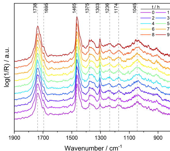
Fig. 2 DRIFT spectra obtained during the induction period at a temperature of 260\text{ }^\circ\text{C} , a \text{H}_2/\text{CO} ratio of 1, 20\text{ cm}^3\text{ min}^{-1} syngas and a pressure of 60 bar.
