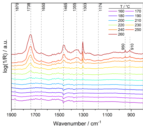
Fig. 1 DRIFT spectra obtained during the heating phase in 20\text{ cm}^3\text{ min}^{-1} syngas with a \text{H}_2/\text{CO} ratio of 1 and a pressure of 60 bar.
