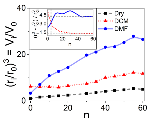
Fig. 4 Average relative volume (r_i/r_0)^3 for the solid support (1% cross-linking, 0.95 mmol \text{g}^{-1} ) relation with the number of repeating units ( n ) from i = 0 to i = n . Dry beads (black squares), compared to swollen particles in DCM (red triangles) and DMF (blue circles); based on the experimental data from Sarin et al. 28 (Table III). In all cases, r_0 refers to the dry original bead. The insert depicts the relative solvent volume increase [(r_i^3 - r_d^3)/r_d^3] comparing the swollen volume to the dry state r_d (red dotted line for DCM and blue continuous line for DMF).
