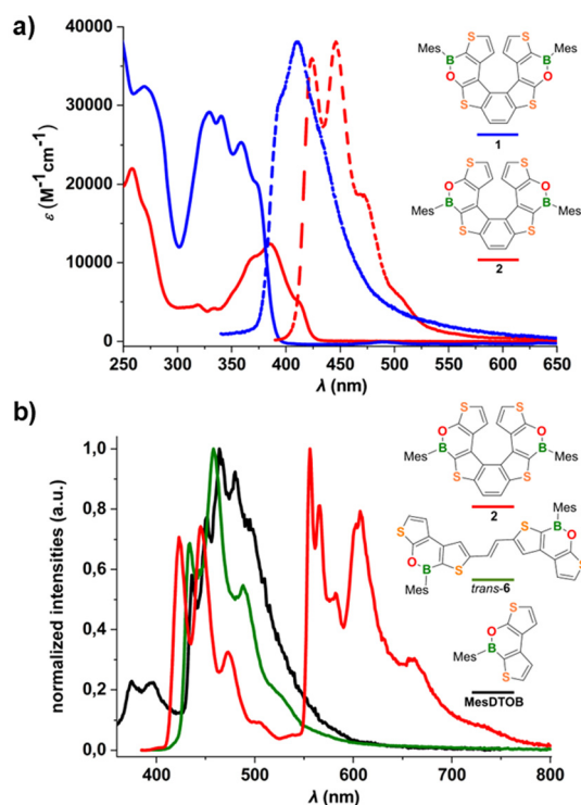
Fig. 5 (a) Molar absorptivity (solid lines) and emission (dashed lines) spectra of 2 (red) and 1 (blue) in c -hexane. (b) Low-temperature emission spectra of 2 (red), trans - 6 (green) and MesDTOB (black) in a frozen toluene matrix (77 K).
