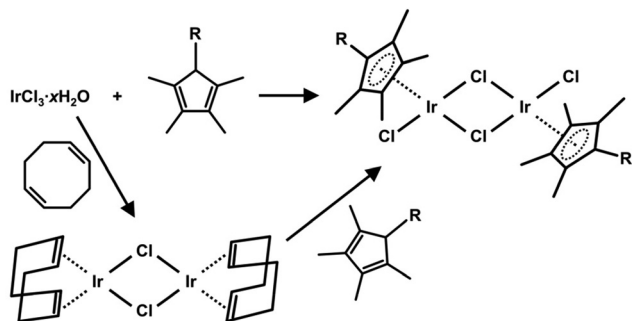
Scheme 1 Synthesis of the most used dinuclear intermediate, [\text{Ir}(\mu\text{-Cl})(\eta^5\text{-Cp}^x)\text{Cl}]_2 , for the synthesis of half-sandwich \text{Ir}(\text{III}) cyclopentadienyl complexes.
