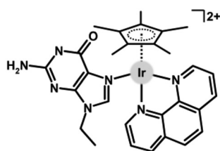
Fig. 43 The structural formula of the adduct of [Ir( \eta^5 -Cp*)(EtG)(phen)] 2+ with 9-ethylguanine (EtG).
