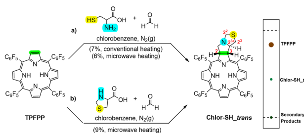
Scheme 1 Synthesis of Chlor-SH trans through 1,3-DC of TPFPP and azomethine ylide generated from paraformaldehyde and (a) cysteine and (b) L -thiazolidine-4-carboxylic acid. TLC representation of the reaction mixture eluted with a mixture of hexane/dichloromethane (6 : 4).
