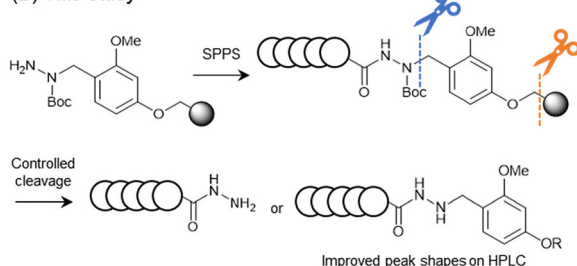
Fig. 1 Various methods for preparing peptide hydrazides.
