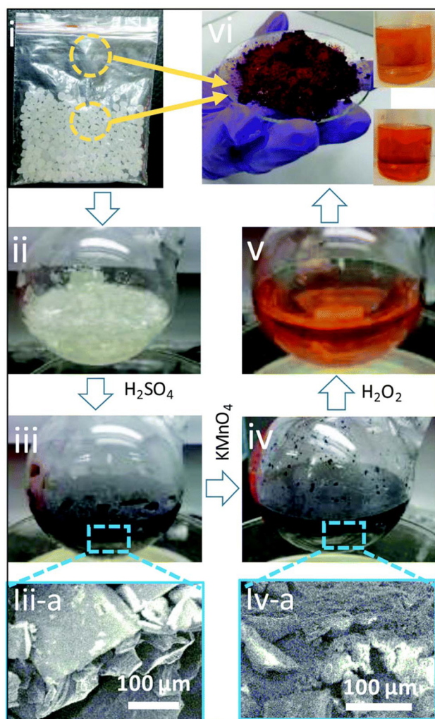
Fig. 1 Photographs showing the transformation from polyethylene into graphitic carbon quantum dots (PE-CQDs). The first step is the acid treatment of PE (i) at \sim 150^\circ\text{C} leading to swelling (ii) and charring (iii). iii-a shows the SEM image of the charred product containing graphitic sheets. \text{KMnO}_4 is added in the second step resulting in a stable black dispersion (iv). The oxidation process leads to functionalization of the graphitic sheets creating a rough surface (iv-a). In the final step, hydrogen peroxide is added into the reaction aliquot yielding an orange-yellow colored stable dispersion of PE-CQDs (v). (vi) Photograph of solid PE-CQDs (5.4 g) obtained from 8 g of polyethylene. Inset images show undisturbed, two-year old PE-CQD solutions in water (bottom) and ethyl acetate (top). Reprinted with permission from ref. 50. Copyright 2020 Royal Society of Chemistry.
