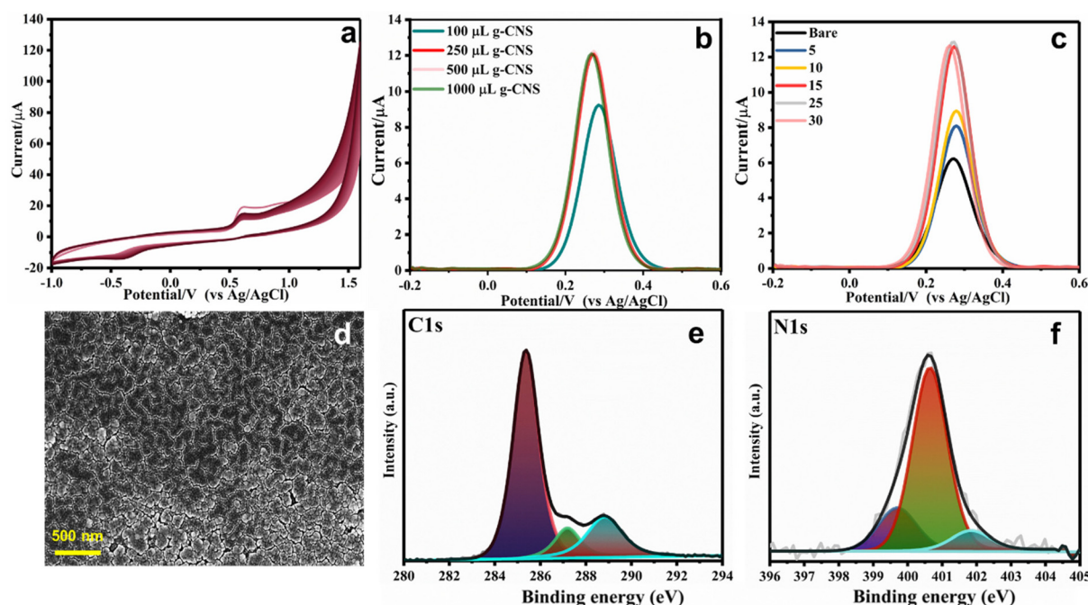
Fig. 4 (a) Electrodeposition cyclic voltammogram of g-CNS on GCE. Comparative SWV current responses of 1 mM K 3 [Fe(CN) 6 ] solution recorded using g-CNS modified with (b) varying concentrations of g-CNS suspension and (c) different numbers of CV cycles. (d) HR-SEM image. (e) C 1s and (f) N 1s XPS spectra of the electrodeposited g-CNS|GCE interface.
