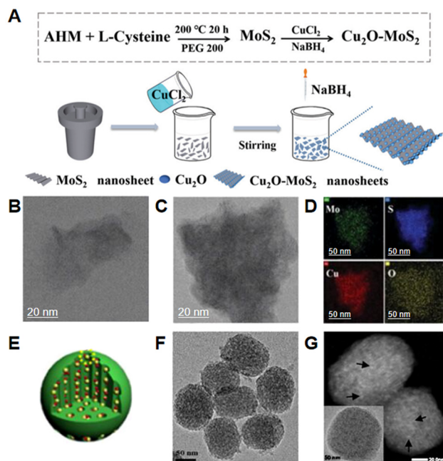
Fig. 8 Preparation and characterization of TMD-oxide composites. (A) Schematic illustration of the synthesis of Cu 2 O-MoS 2 . (B) TEM images of (B) MoS 2 and (C) Cu 2 O-MoS 2 . (D) Elemental mapping images of Mo, S, Cu, and O. 88 Reproduced with permission from ref. 88. Copyright 2021 Royal Society of Chemistry. (E) Structural sketch, (F) TEM, and (G) STEM images of UsMSND@MSN. Inset: enlarged TEM image of an individual UsMSND@MSN nanoparticle. 89 Reproduced with permission from ref. 89. Copyright 2021 Elsevier.
