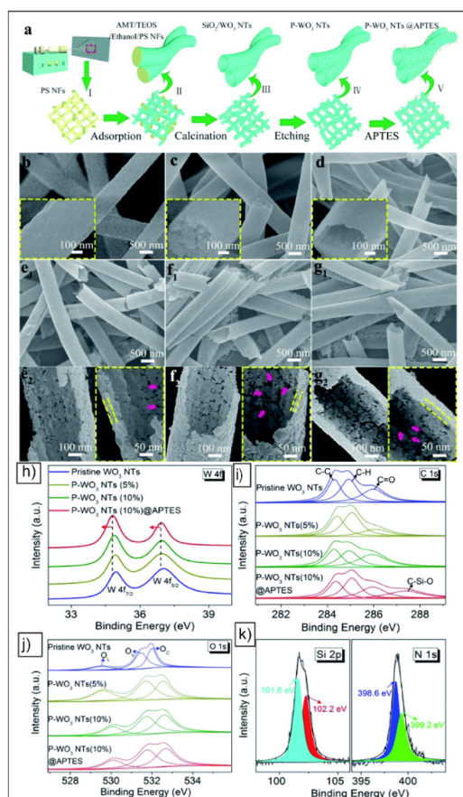
Fig. 10 (a) Schematic of the synthetic process for APTES functionalized porous \text{WO}_3 NTs. The SEM images of the (b) as-spun PS nanofibers, (c) AMT/TEOS/PS composite nanofibers, and (d) \text{SiO}_2/\text{WO}_3 composite NTs. (e 1 ) SEM image and (e 2 ) corresponding magnifications of P- \text{WO}_3 NTs (5%). (f 1 ) SEM image and (f 2 ) corresponding magnifications of P- \text{WO}_3 NTs (10%). (g 1 ) SEM image and (g 2 ) corresponding magnifications of P- \text{WO}_3 NTs (10%)@APTES. The inset images in panels (b), (c) and (d) are the corresponding magnifications. (h) W 4f, (i) C 1s, and (j) O 1s XPS spectra of the pristine \text{WO}_3 NTs, P- \text{WO}_3 NTs (5%), P- \text{WO}_3 NTs (10%) and P- \text{WO}_3 NTs (10%)@APTES samples. (k) Si 2p and N 1s XPS spectra of the P- \text{WO}_3 NTs (10%)@APTES sample. Reproduced from ref. 47 with permission from RSC, copyright 2018.
