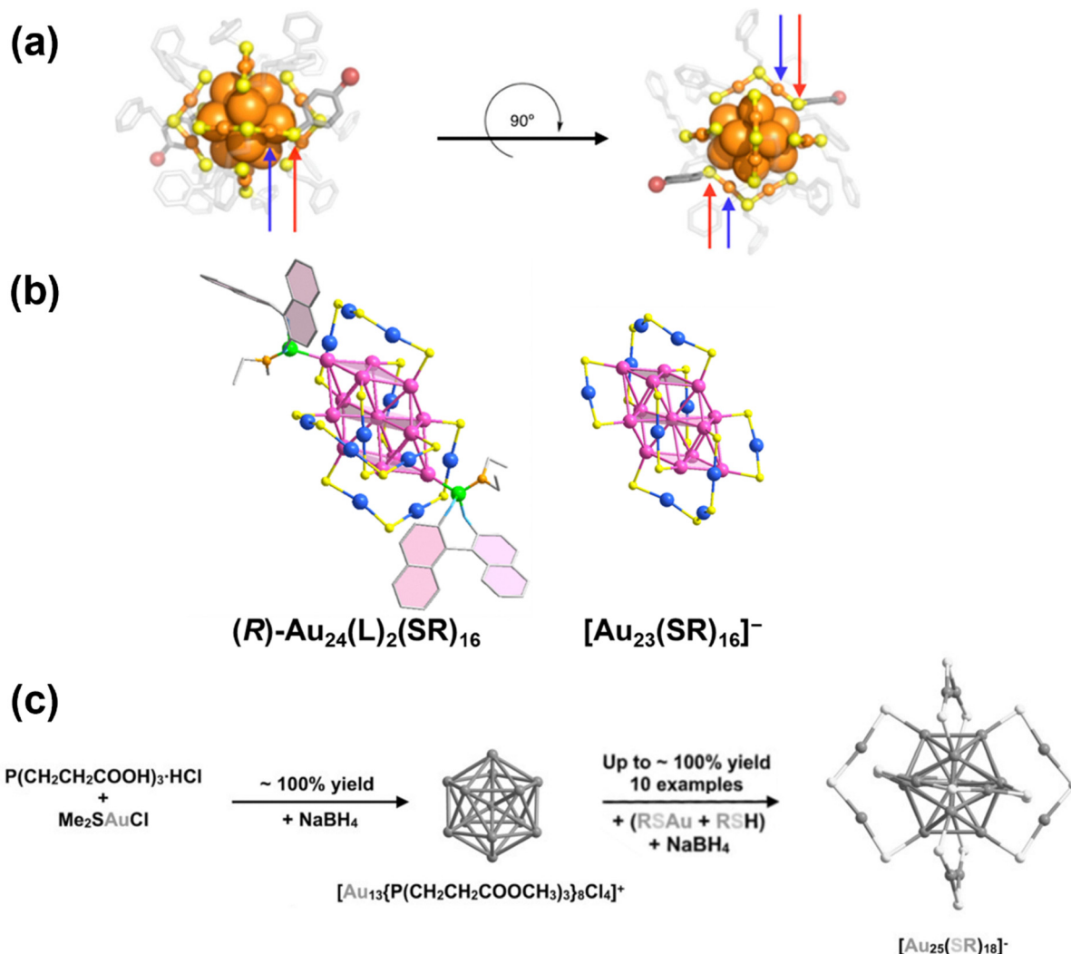
Fig. 11 (a) Structure of Au 25 (PET) 18 ( p -BBT) 2 ( p -BBT = 4-bromobenzenethiol) resolved by SCXRD. Colour label: orange, Au; yellow, S; grey, C; red, Br. Red arrows indicate the locations of exchanged p -BBT ligands and blue arrows indicate the Au atoms on the surface motif that bond to the exchanged p -BBT ligands. Reprinted with permission from ref. 195. Copyright 2014, American Chemical Society. (b) The total structures of [Au 23 (S- c -C 6 H 11 ) 16 ] - after ( R configuration) and before the exchange reaction with phosphoramidite. Colour label: pink, core Au; blue, motif Au; yellow, S; green, P; orange, N; light blue, O; grey, C. Reprinted with permission from ref. 8. Copyright 2023, Springer Nature Limited. (c) Schematic illustration of the reaction process of the seeded growth of [Au 25 (SR) 18 ] - . Reprinted with permission from ref. 197. Copyright 2021, Wiley-VCH.
