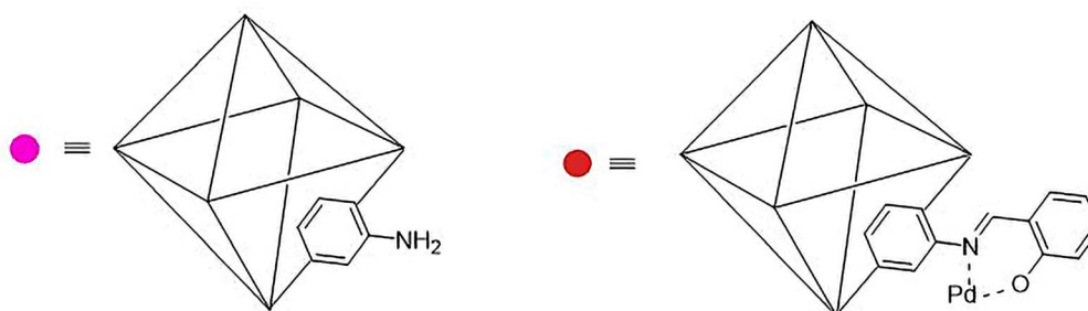
Scheme 1 Preparation of \text{Fe}_3\text{O}_4@\text{MCM-41}@UiO-66/\text{SB-Pd} .
