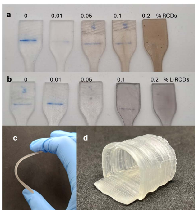
Fig. 4 Samples of dog-bones (after tensile tests) printed with Resin-F containing increasing amounts of RCDs (a) and L-RCDs, (b) (0, 0.01, 0.05, 0.1 and 0.2% w/w); (c) flexibility of F@L-RCDs-0.2%; (d) a trachea printed with Resin-F@L-RCDs-0.2%.
