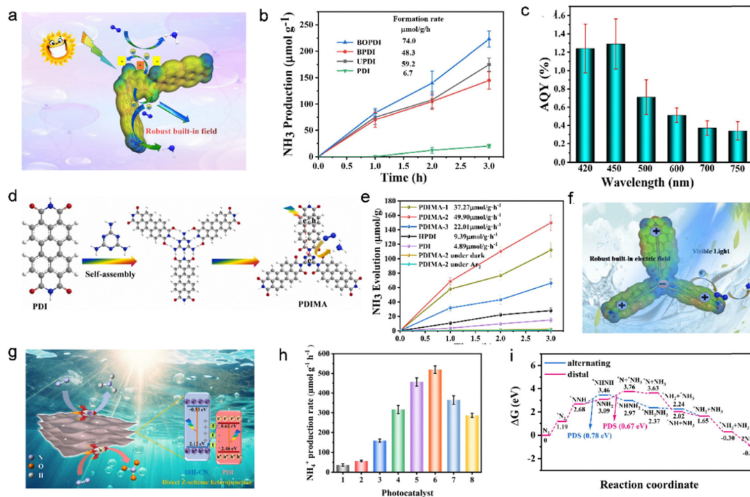
Fig. 17 (a) Plausible mechanism for the photocatalytic \text{N}_2 fixation over BOPDI under visible light irradiation. (b) \text{NH}_3 evolution rates over the as-prepared BOPDI catalysts. (c) Apparent quantum efficiency (AQY) of BOPDI. Reproduced from ref. 159. Copyright 2022, Elsevier. (d) Schematic diagram of the synthetic route. (e) Ammonia synthesis rates over different samples. (f) Diagram of the photocatalytic nitrogen fixation mechanism over PDIMA-2. Reproduced from ref. 160. Copyright 2022, Elsevier. (g) Direct Z-scheme heterojunction of 10H-CNv. (h) Average \text{NH}_4^+ yields for different photocatalysts. (i) Gibbs free energy diagrams of the photocatalytic reduction of ammonia by \text{N}_2 in 30% PDI/10H-CNv composites. Reproduced from ref. 161. Copyright 2024, Elsevier.
