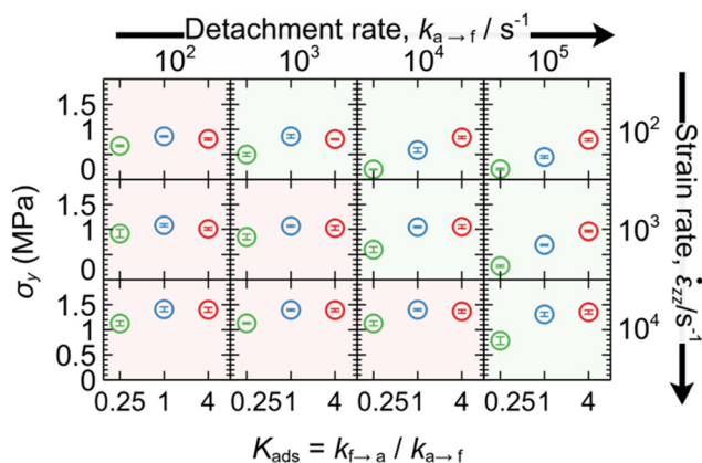
Fig. 12 Yield stress \sigma_y as a function of the detachment rate k_{a \rightarrow f} , elongation rate \dot{\epsilon}_{zz} and adsorption constant K_{\text{ads}} = k_{f \rightarrow a}/k_{a \rightarrow f} = 1/4 (green), 1 (blue) and 4 (red). Scenarios where \dot{\epsilon}_{zz} is smaller (larger or equal) than k_{a \rightarrow f} are indicated with green (red) background. The error bars correspond to the standard deviation from three individual experiments.
