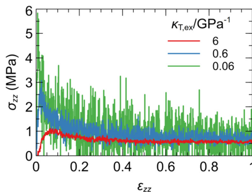
Fig. 13 Stress–strain curve from a tack experiment with \dot{\epsilon}_{zz} = k_{a \rightarrow f} = 10^5 \text{ s}^{-1} and K_{\text{ads}} = 1 . Red curve illustrates a case using the default parameters in Table 1. Blue/green curve illustrates the impact of decreasing compressibility by a factor of 10/100 upon multiplying the characteristic pressure P^* by 10/100, respectively.
